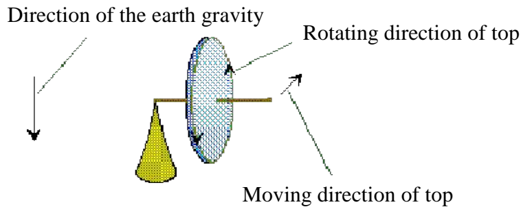
Fig. 3.1 Motion of a top which axis of rotation is leveled
