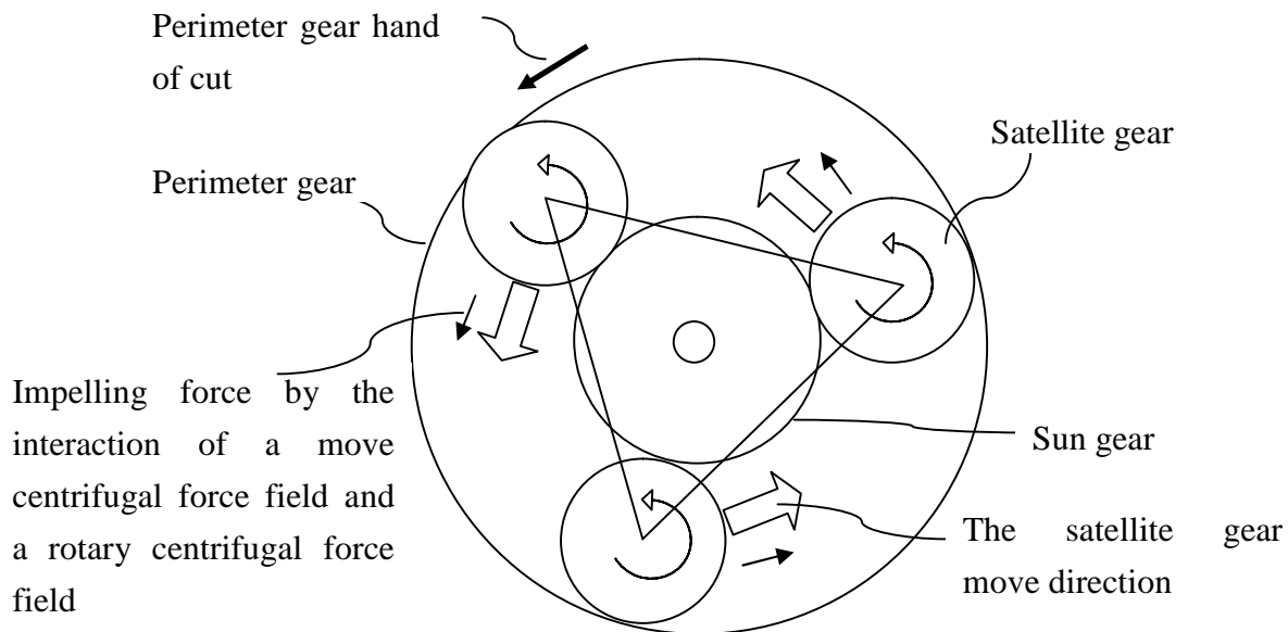
Fig. 4.2 The planetary gear mechanism in consideration of the direction of impelling force of the centrifugal force interaction
