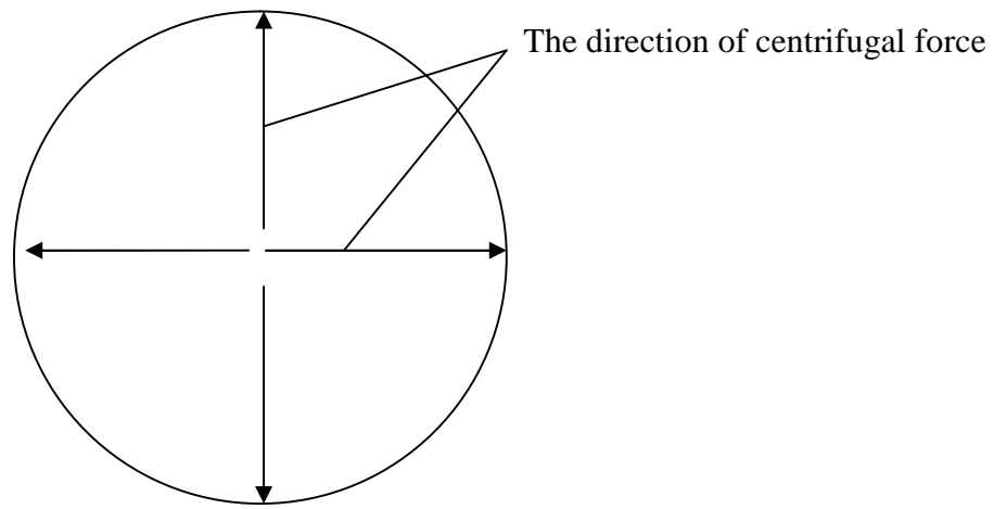
Fig. 2.1 The direction of the centrifugal force observed from the rotating coordinate system
