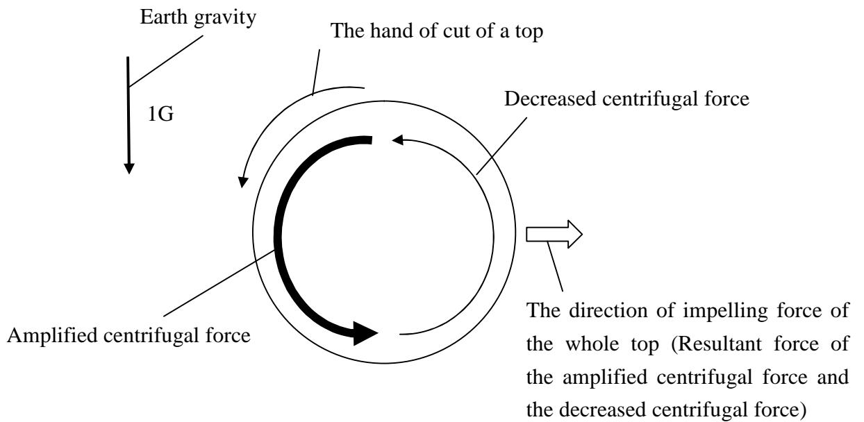
Fig. 3.2 Composition of earth gravity and centrifugal force
