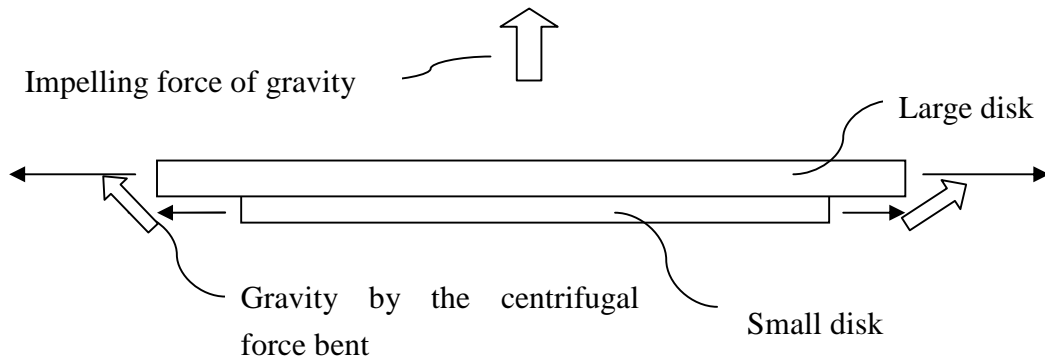
Fig.5.2 Gravity by the centrifugal force bent
