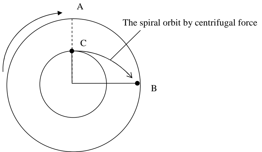
Fig. 2.2 The direction of the centrifugal force observed from the non-rotating coordinate system
