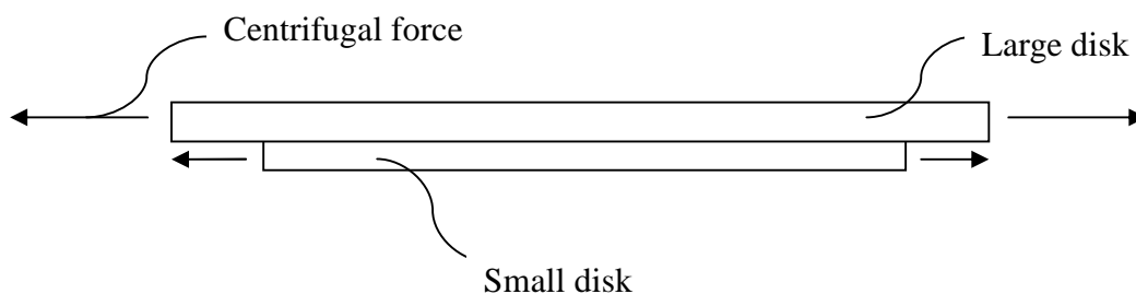
Fig.5.1 Contiguity of the big partial gravitational field of centrifugal force, and a little small partial gravitational field
