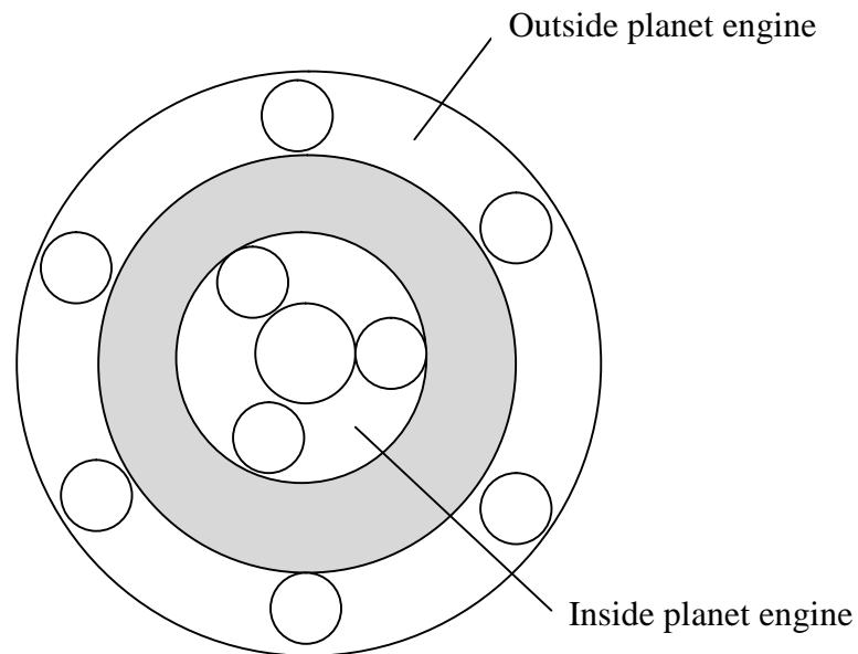
Fig. 6.1 The direction control of gravity impelling force with two planet engines
