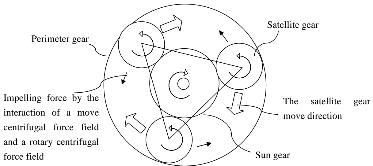
Fig. 4.1 The direction of impelling force of an ordinary planetary gear mechanism and its centrifugal force interaction
